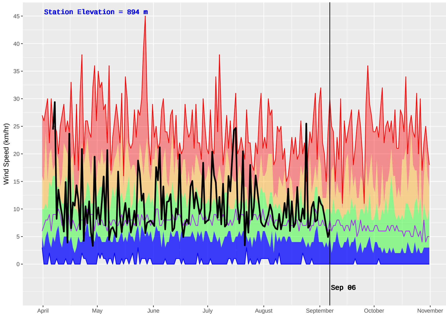
TOBY HUB (417) : Historical (1986–2016) and Current (2017) Noon Wind Speed
