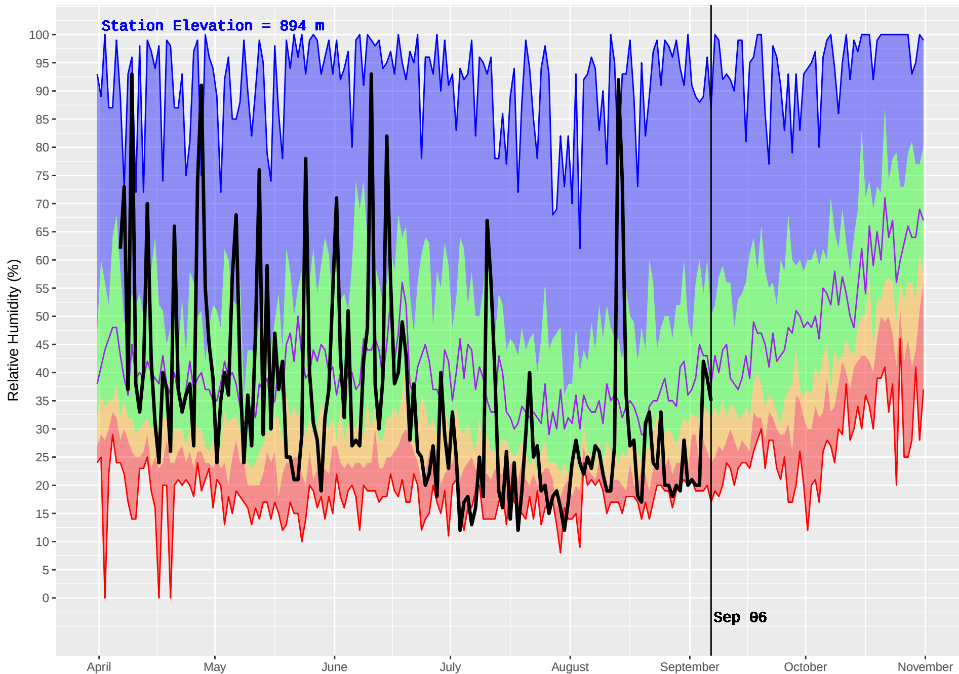
TOBY HUB (417) : Historical (1986–2016) and Current (2017) Noon Relative Humidity
