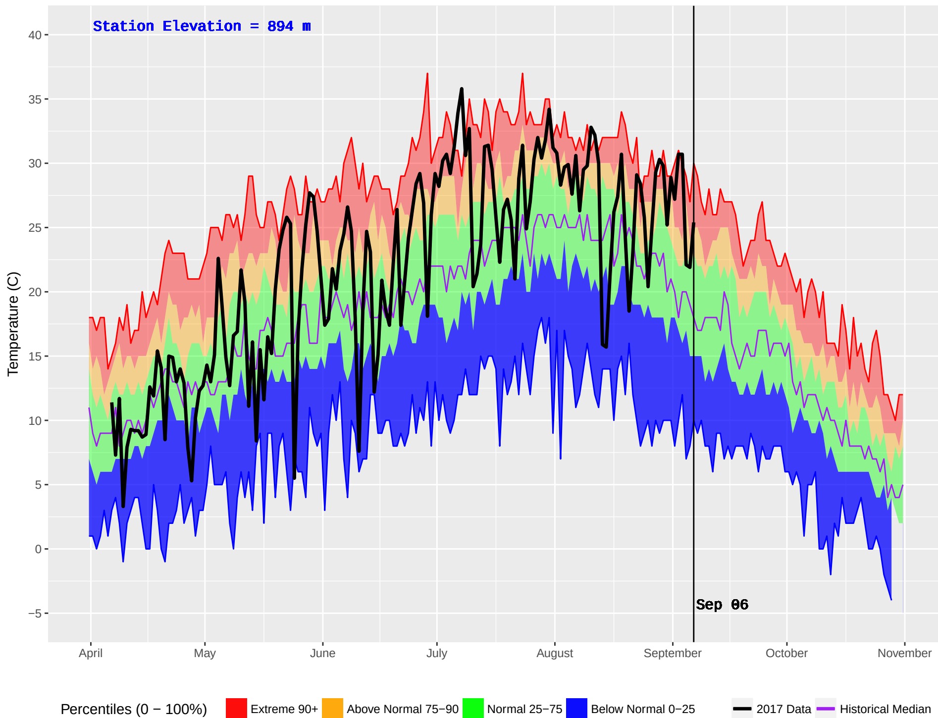
TOBY HUB (417) : Historical (1986–2016) and Current (2017) Noon Temperature
